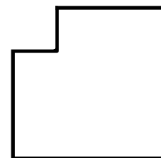
Hexagon – Square with corner cut out
