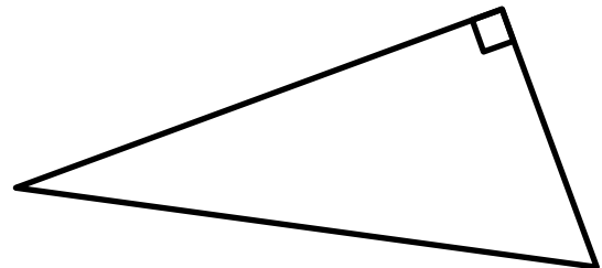
Scalene right-angled triangle
