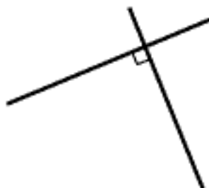
Right angle
