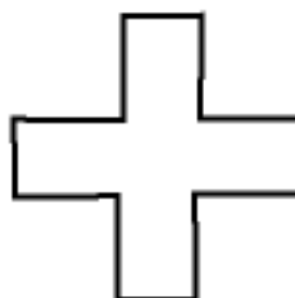
Dodecagon - Cross
