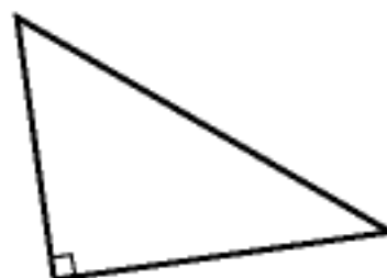
Right angled triangle
