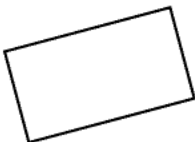
Rectangle
