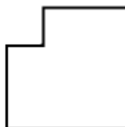
Square with corner cut out
