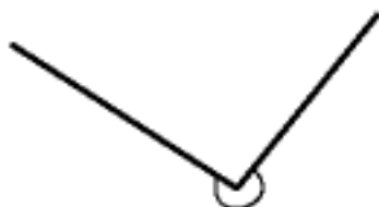
Reflex angle
