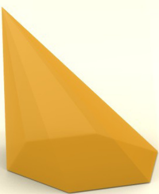
Hexagonal Pyramid
