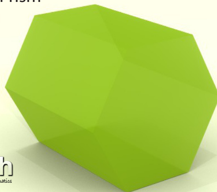
Hexagonal Prism
