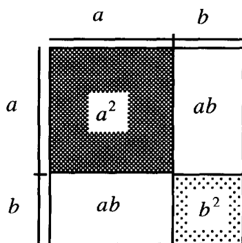
Figure 1. (a + b)^2 = a^2 + 2ab + b^2
